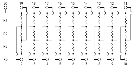
830 ELECTRICAL SCHEMATIC
