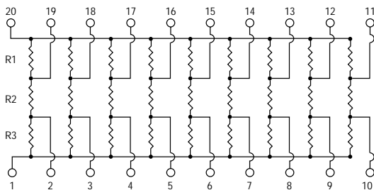
820 ELECTRICAL SCHEMATIC
